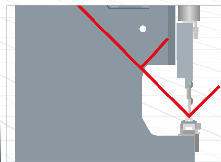
90° Endless Bend
